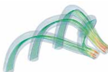
The Stream toolset in Abaqus enables users to visualize fluid flow data by placing a rake, or a line segment with a number of points specified along its length, allowing the display of fluid flow in the model.
