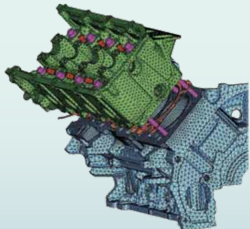
Abaqus offers a sophisticated environment for accelerating contact modeling and mesh creation. Image courtesy of Ford Motor Company
